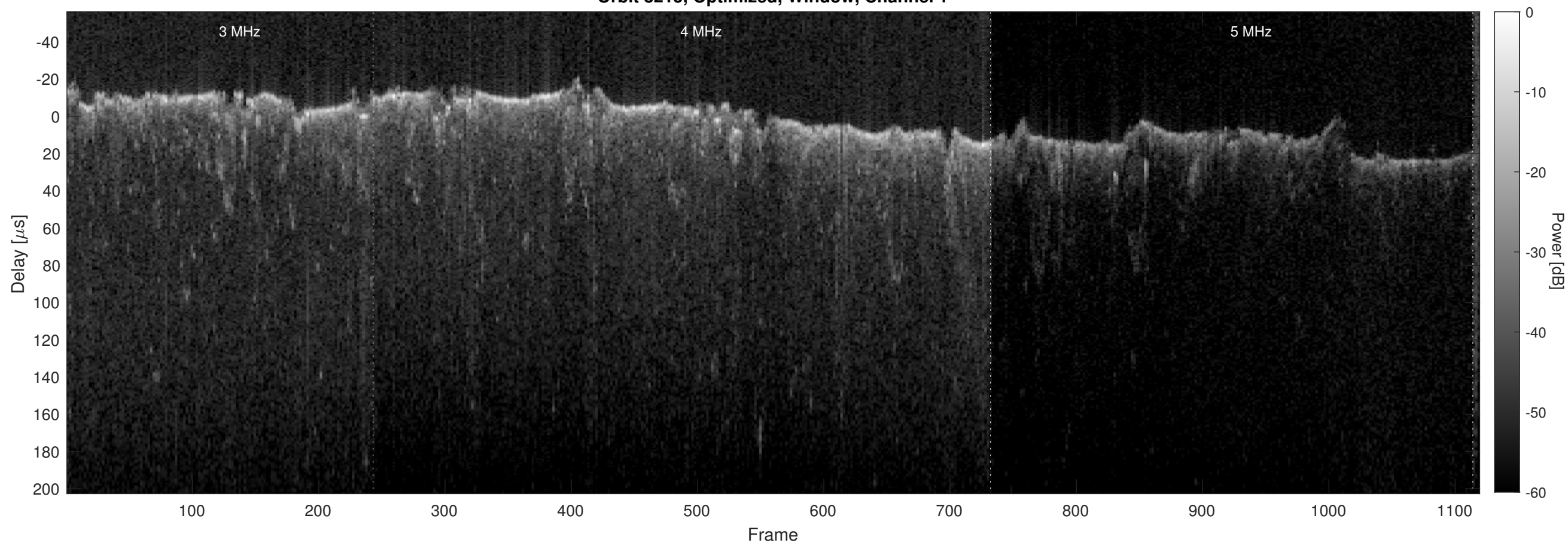
Orbit 8215, Optimized, Window, Channel 2
