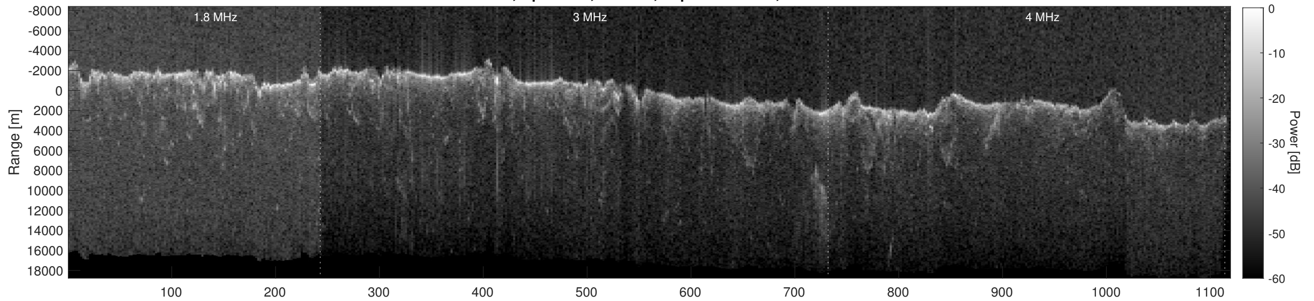
Orbit 8215, Depth-Corrected Cluttergram
