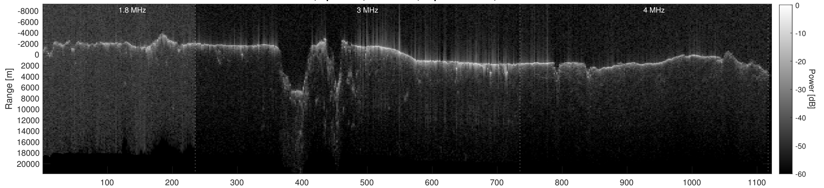
Orbit 8216, Depth-Corrected Cluttergram
