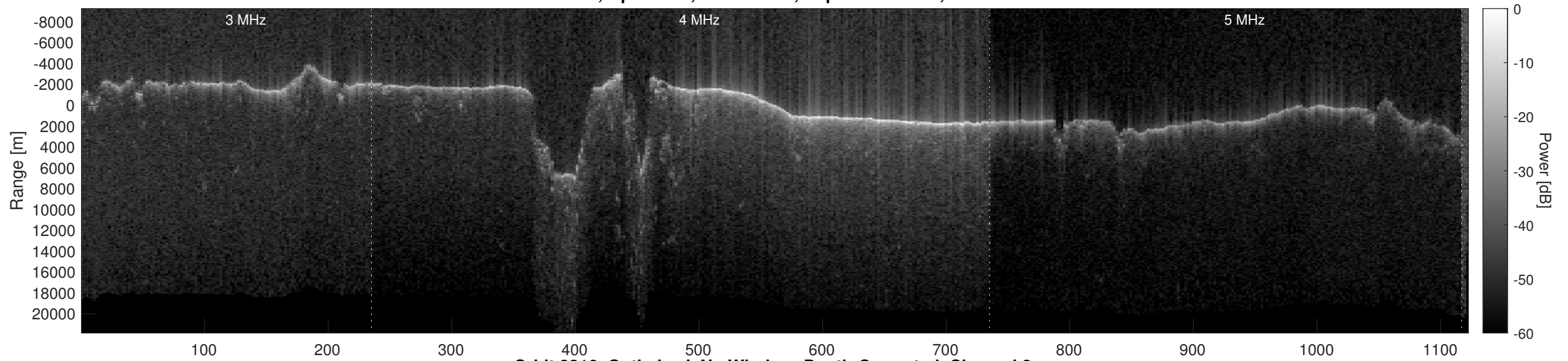
Orbit 8216, Optimized, No Window, Depth-Corrected, Channel 2
