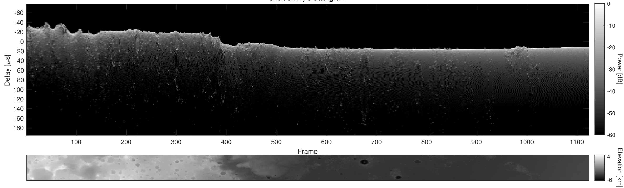
Orbit 8217, Cluttergram
