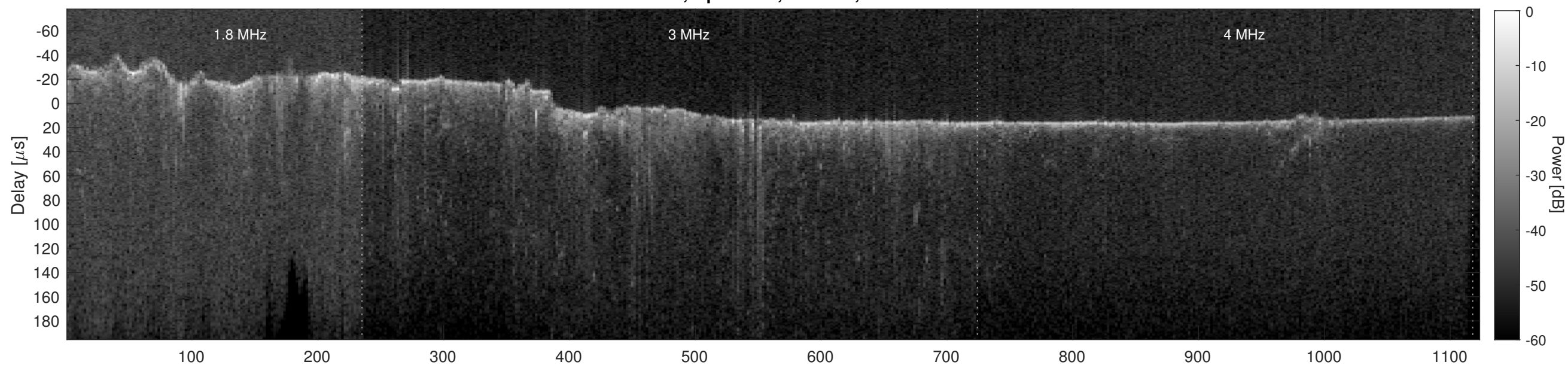
Orbit 8217, Cluttergram
