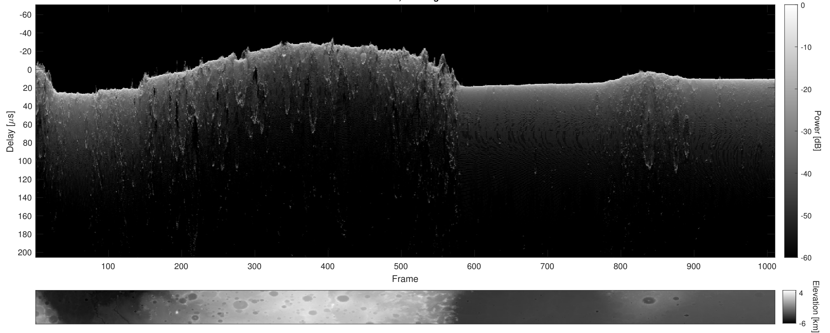
Orbit 8218, Cluttergram
