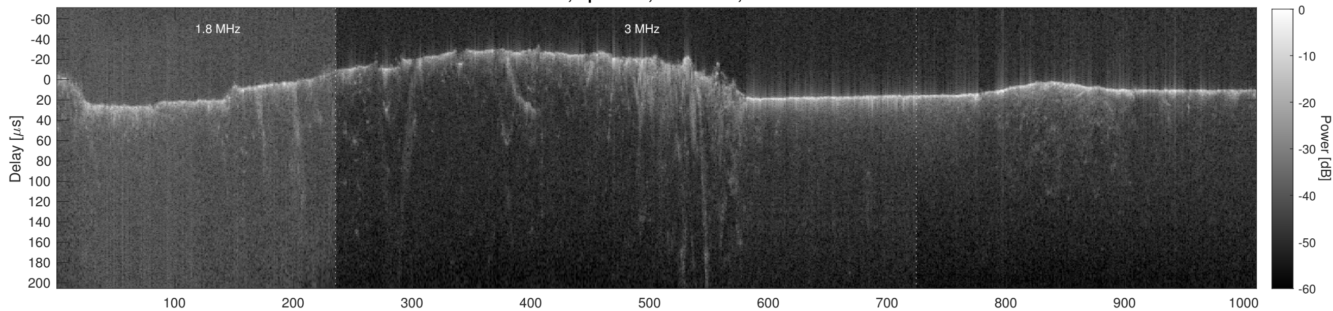
Orbit 8218, Cluttergram
