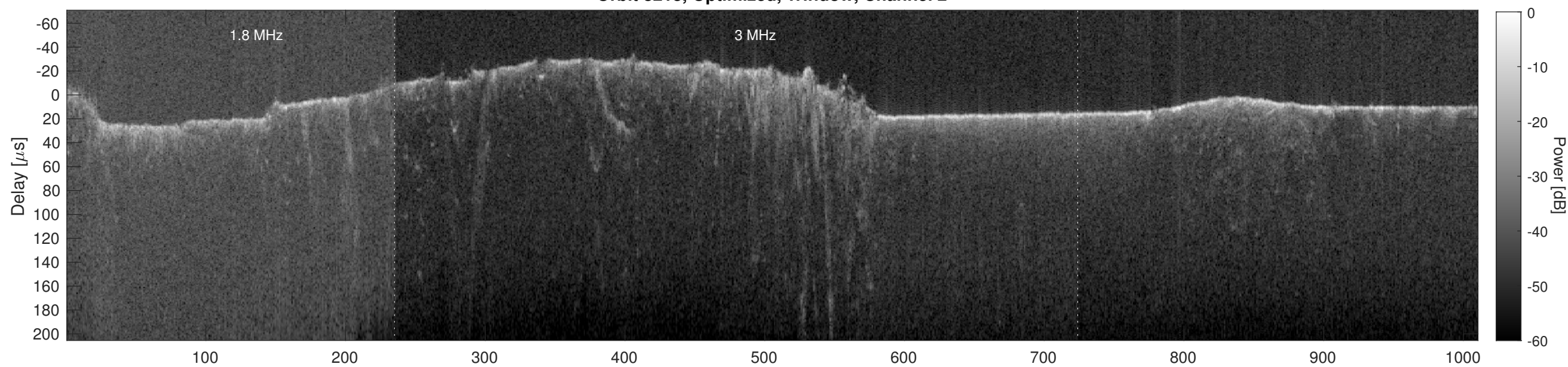
Orbit 8218, Cluttergram
