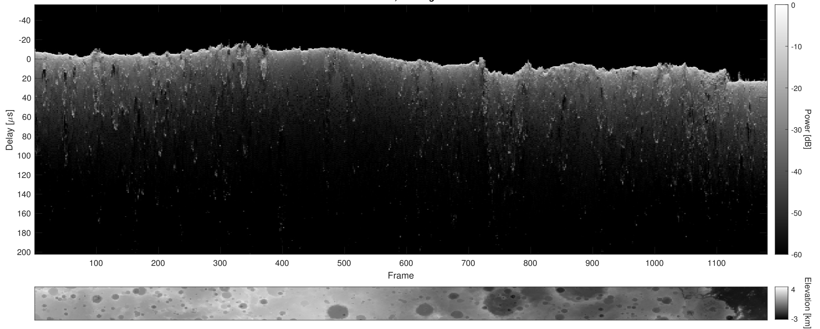
Orbit 8222, Cluttergram
