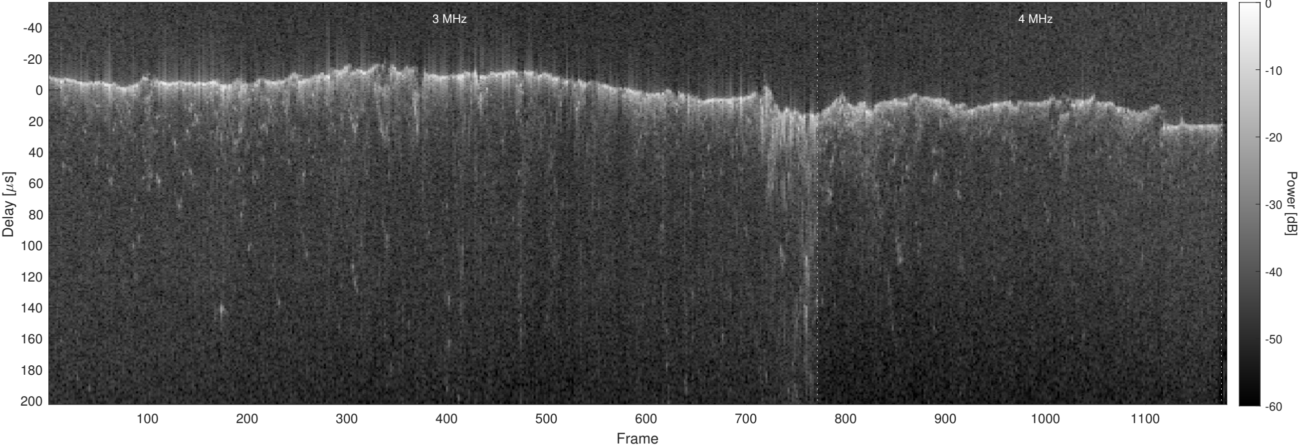
Orbit 8222, Optimized, No Window, Channel 2
