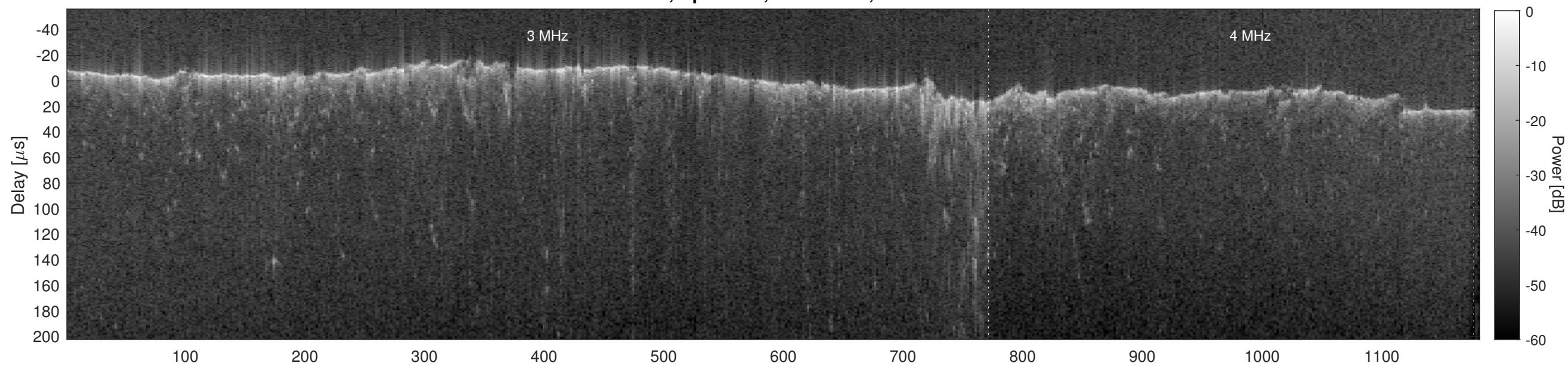
Orbit 8222, Cluttergram
