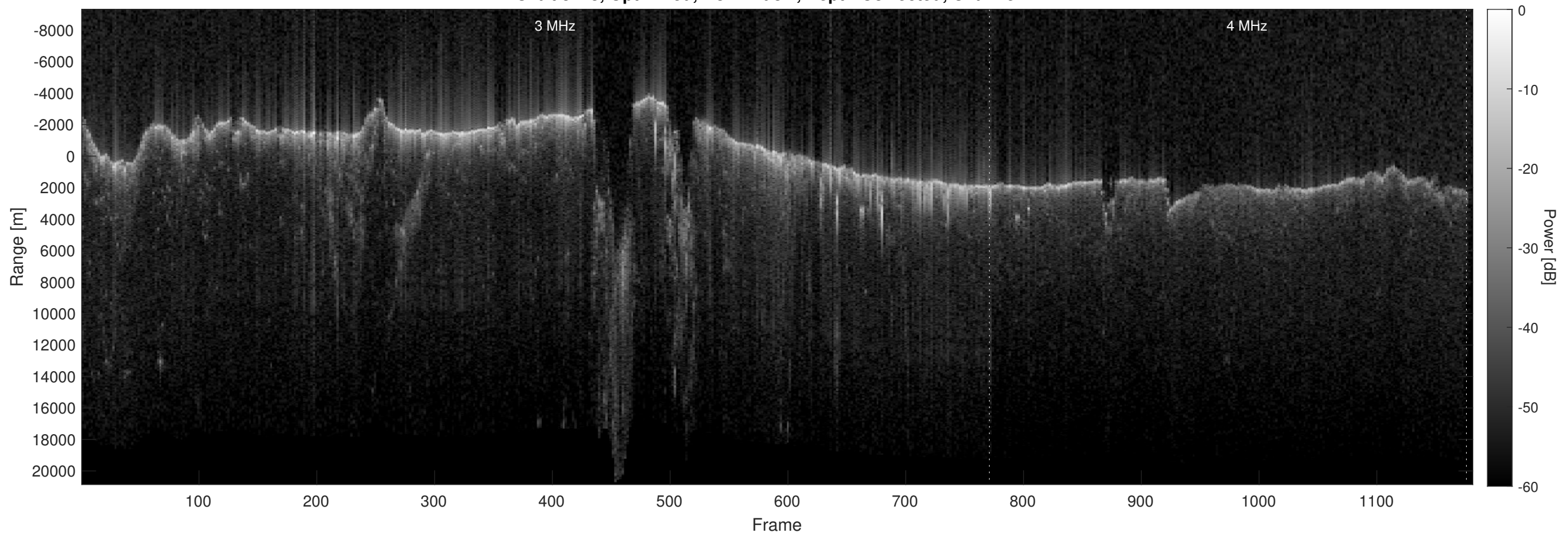
Orbit 8223, Optimized, No Window, Depth-Corrected, Channel 2
