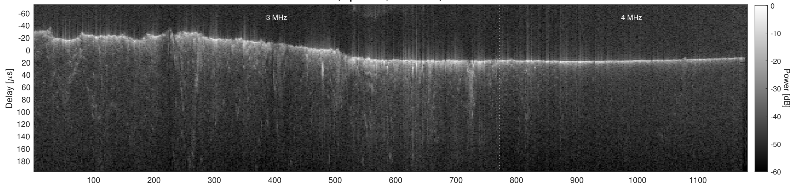
Orbit 8224, Cluttergram
