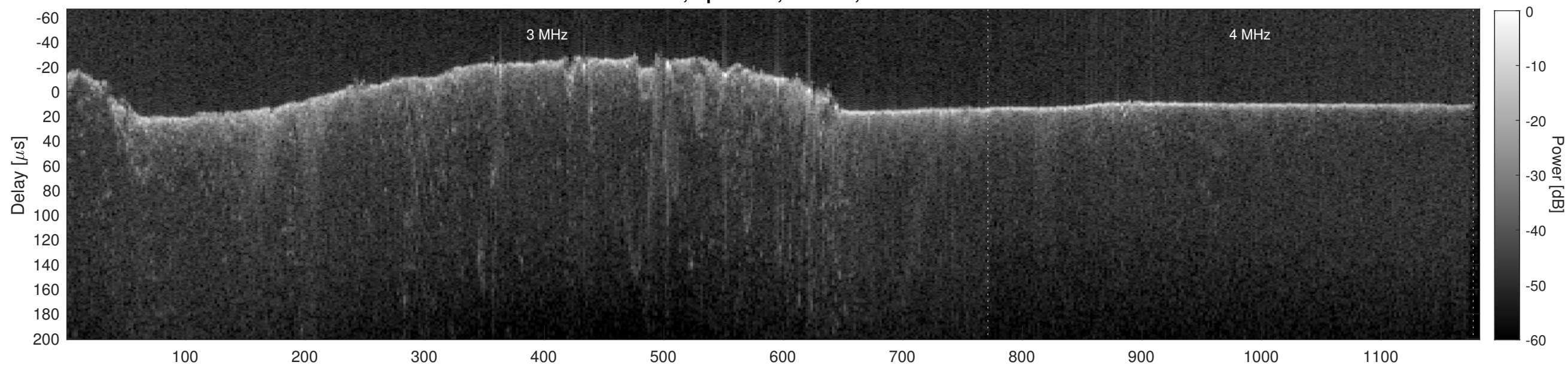
Orbit 8225, Cluttergram
