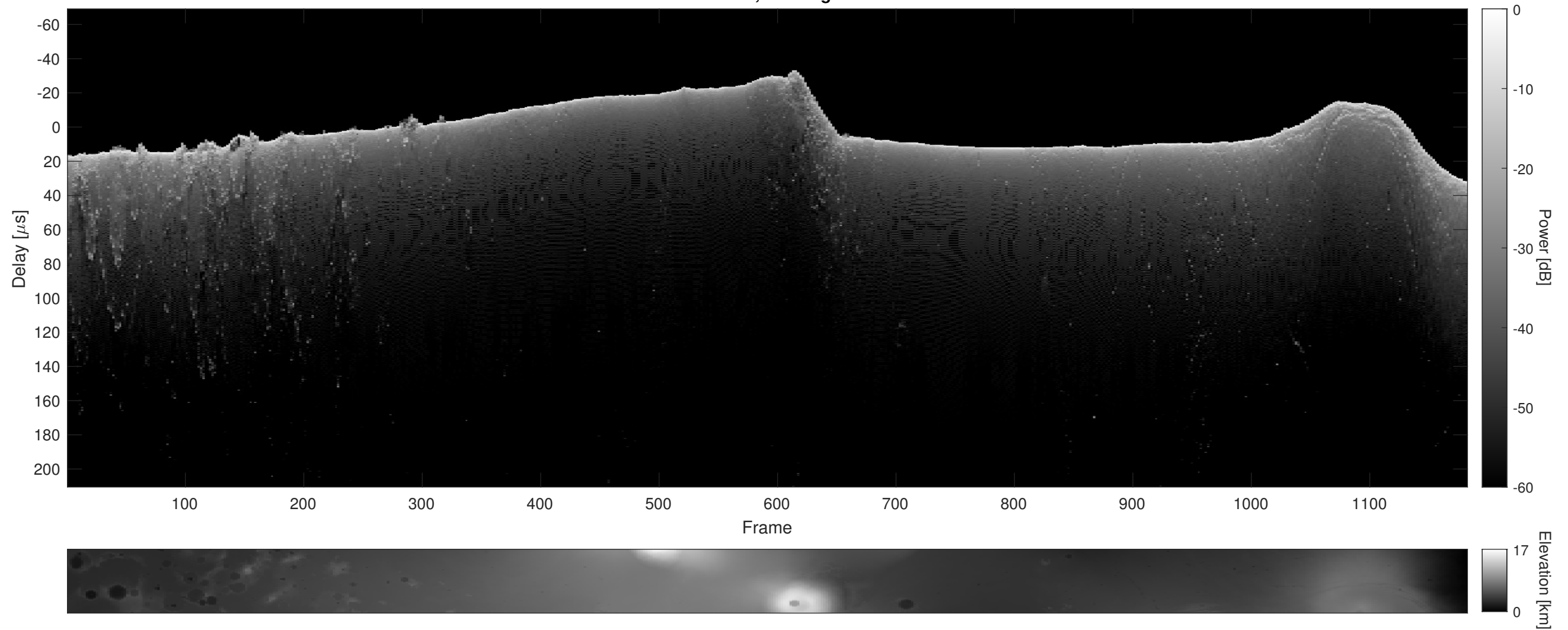
Orbit 8227, Cluttergram
