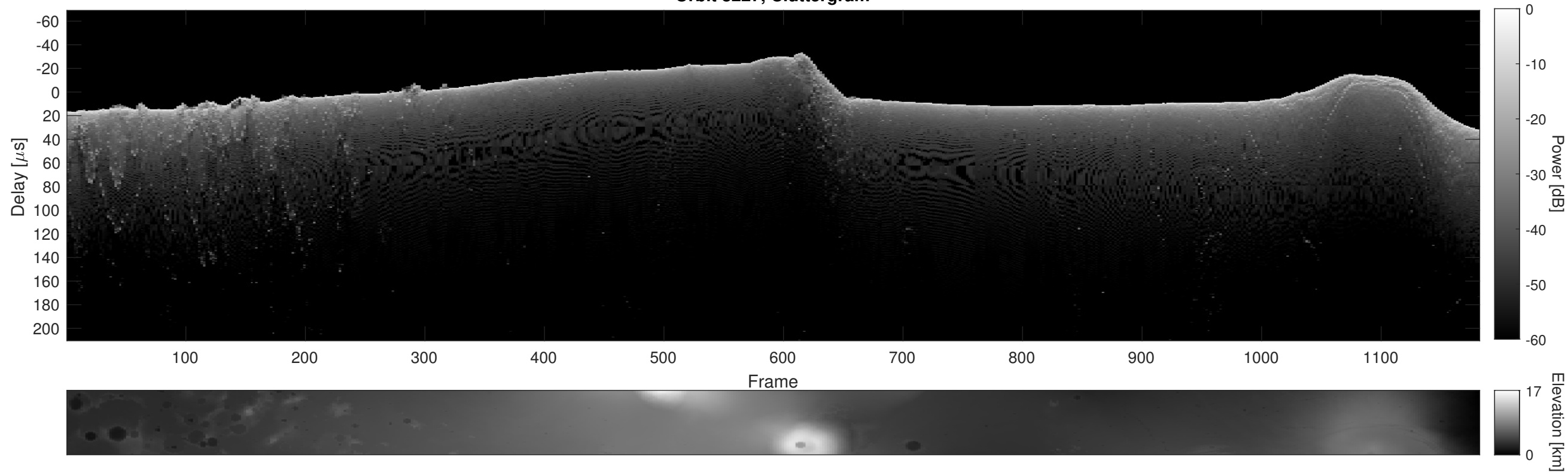
Orbit 8227, Cluttergram
