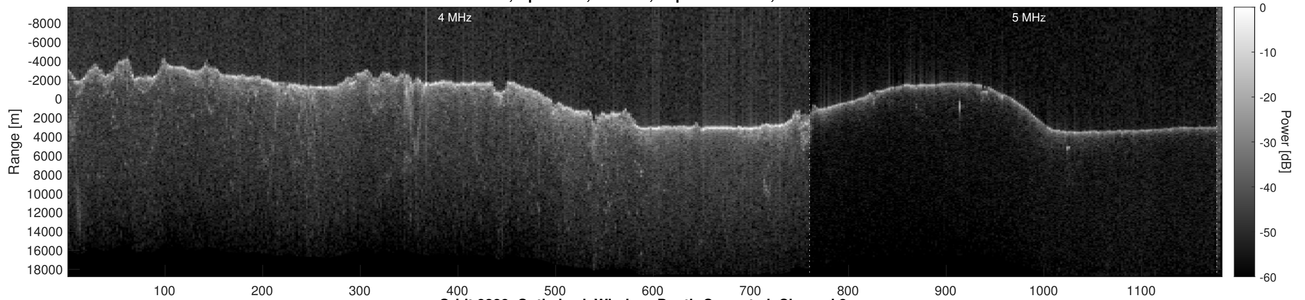
Orbit 8228, Optimized, Window, Depth-Corrected, Channel 2
