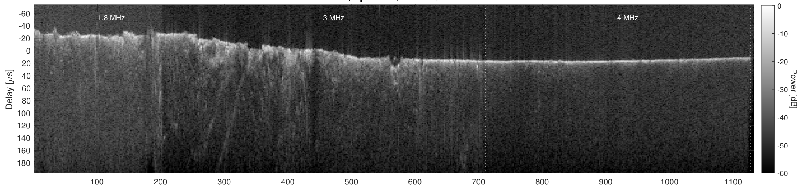
Orbit 8231, Cluttergram
