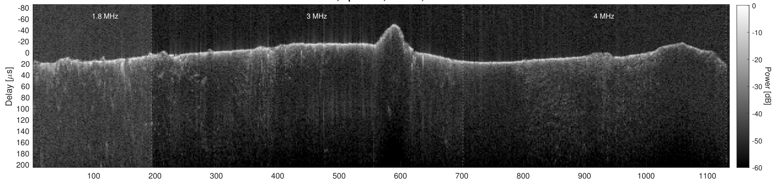
Orbit 8234, Cluttergram
