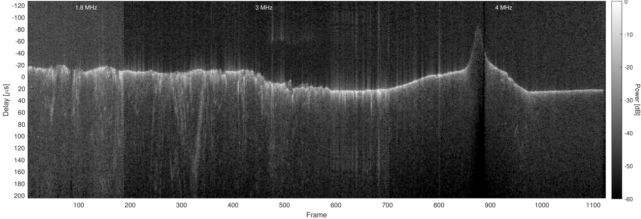
Orbit 8235, Optimized, No Window, Channel 2
