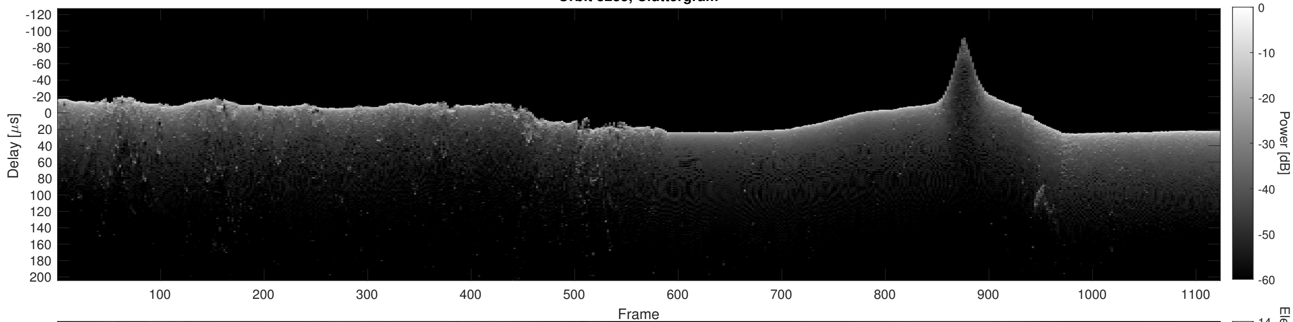
Orbit 8235, Cluttergram
