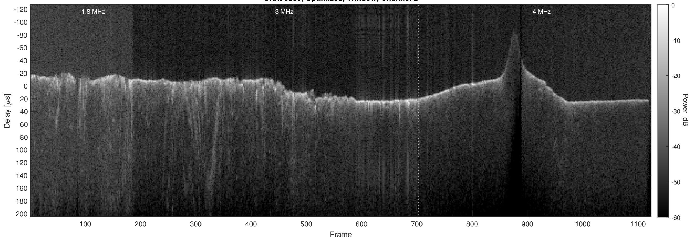
Orbit 8235, Optimized, Window, Channel 2
