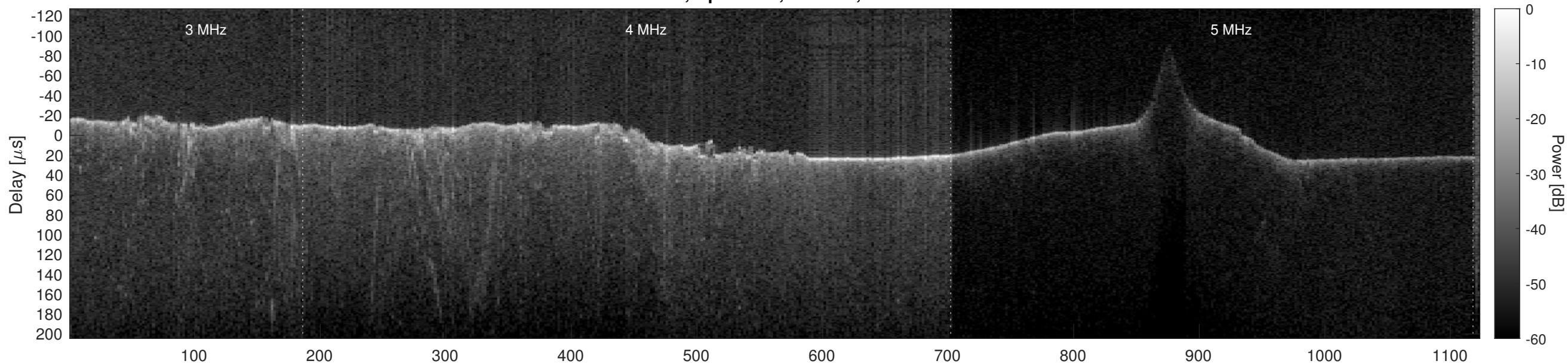
Orbit 8235, Optimized, Window, Channel 2
