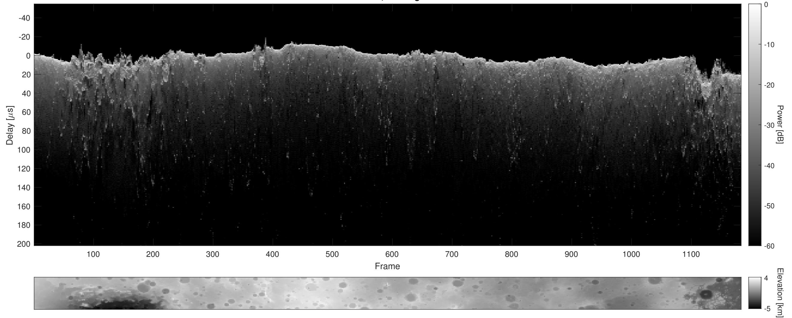
Orbit 8236, Cluttergram
