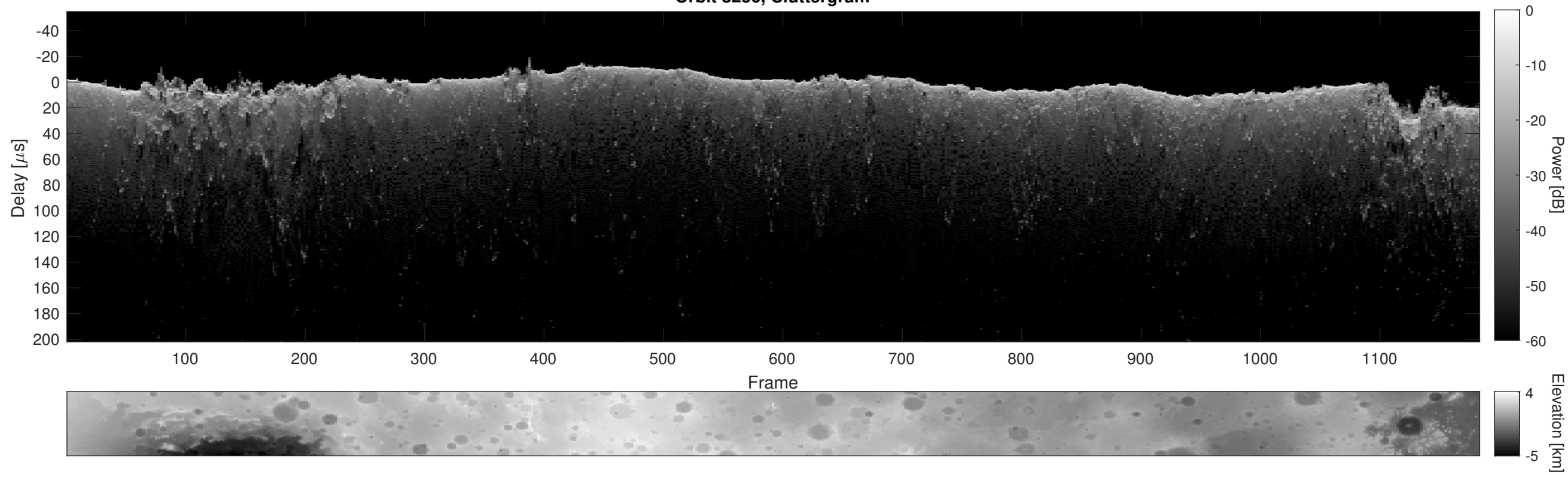
Orbit 8236, Cluttergram
