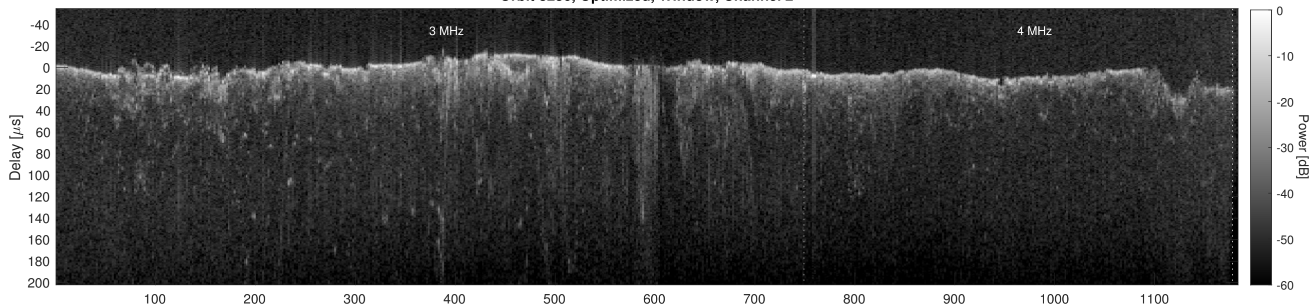
Orbit 8236, Cluttergram
