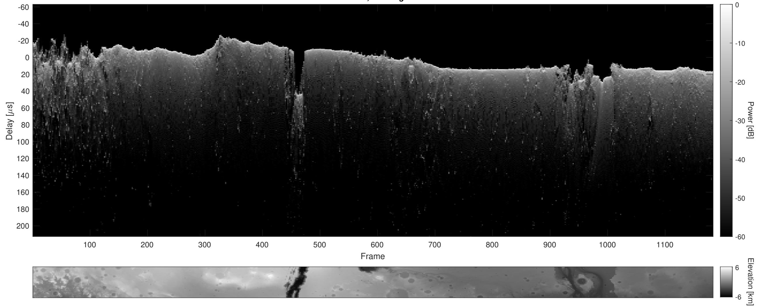
Orbit 8237, Cluttergram
