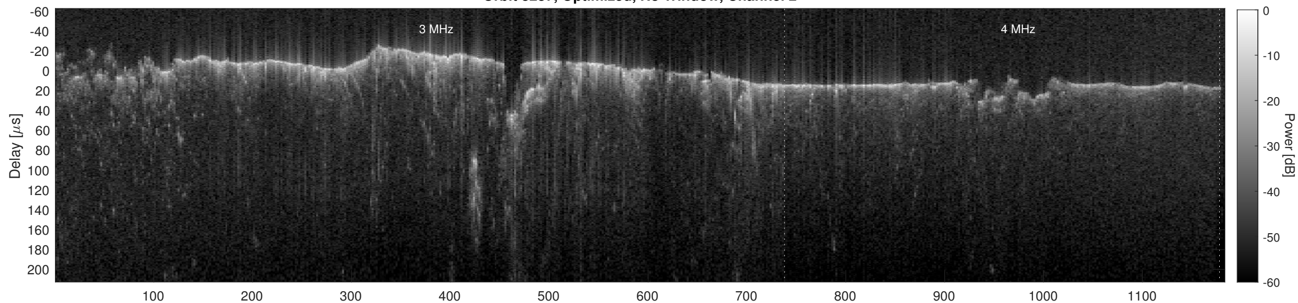
Orbit 8237, Cluttergram
