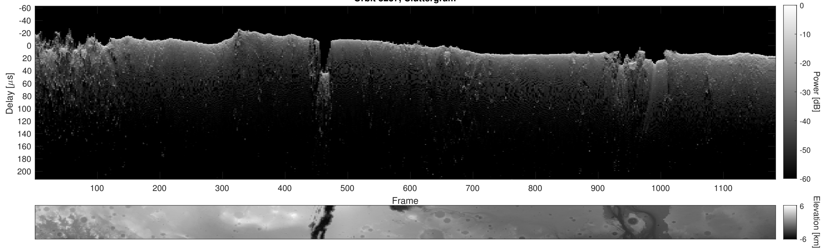
Orbit 8237, Cluttergram
