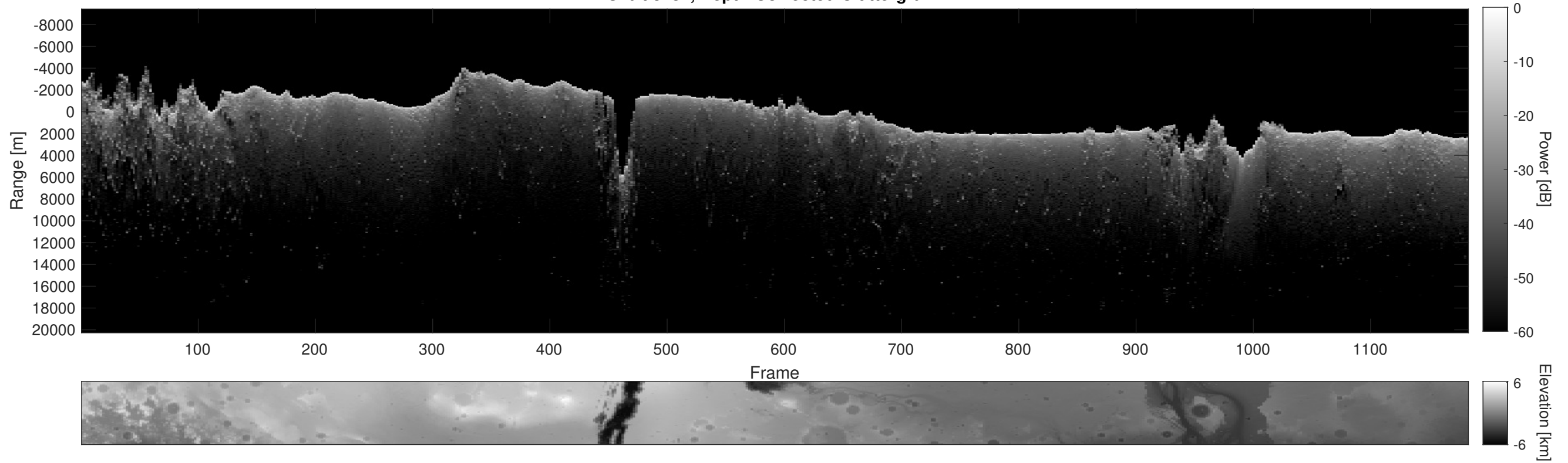
Orbit 8237, Depth-Corrected Cluttergram
