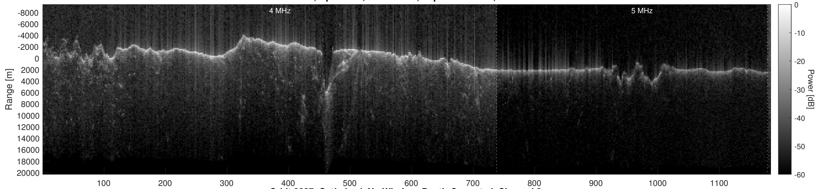
Orbit 8237, Optimized, No Window, Depth-Corrected, Channel 2
