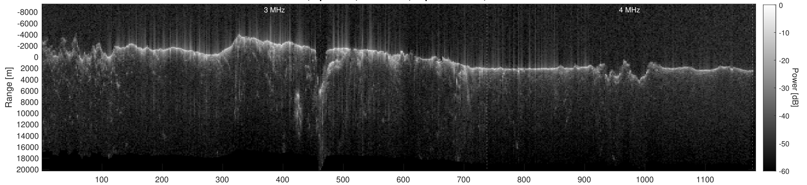
Orbit 8237, Depth-Corrected Cluttergram
