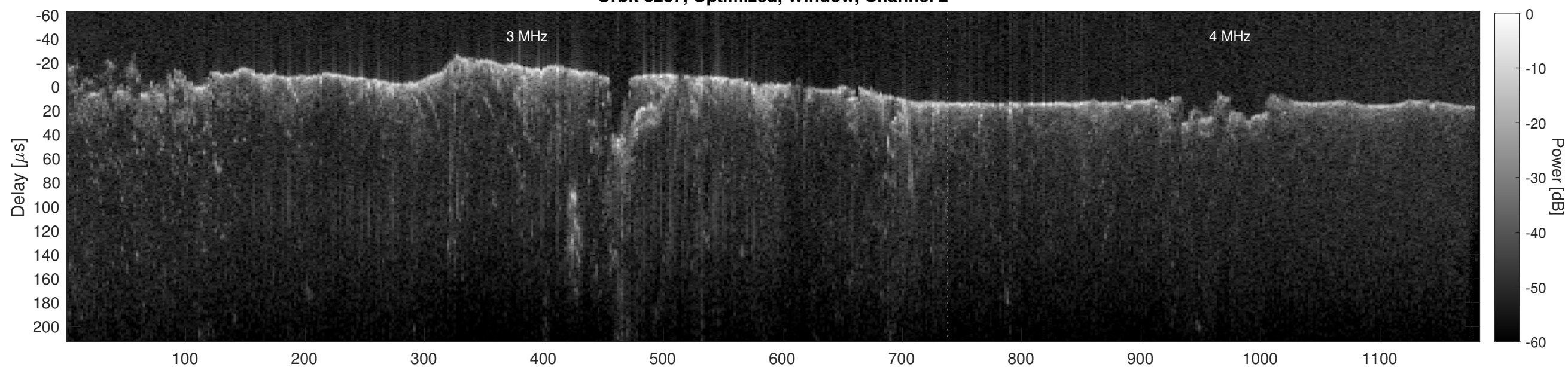
Orbit 8237, Cluttergram
