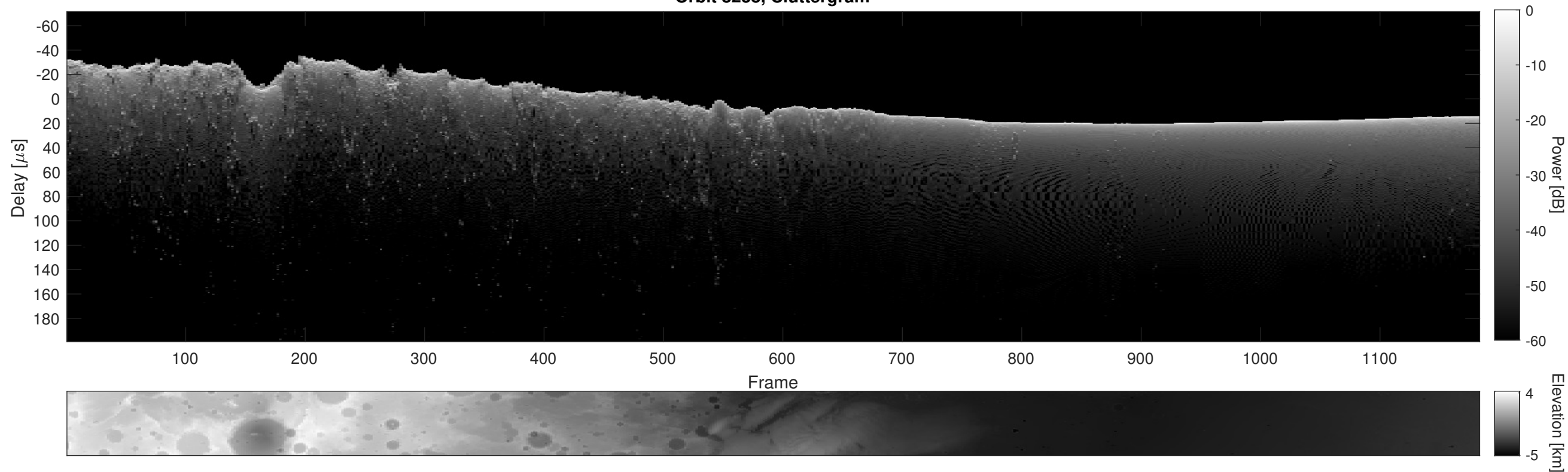
Orbit 8238, Cluttergram
