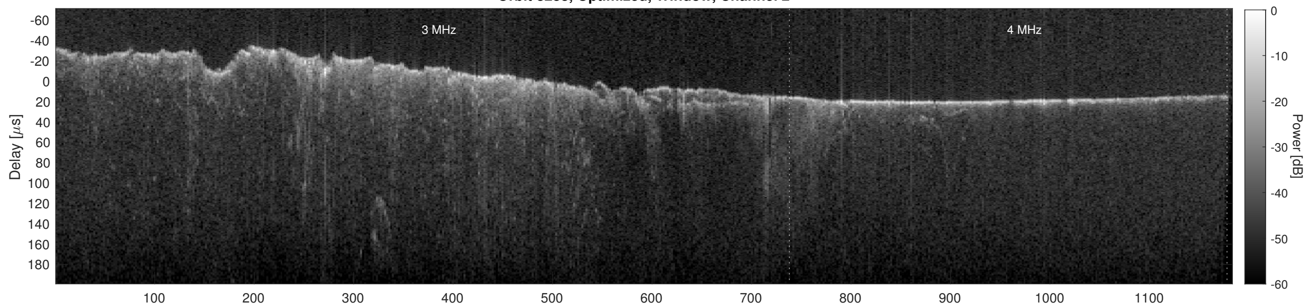
Orbit 8238, Cluttergram
