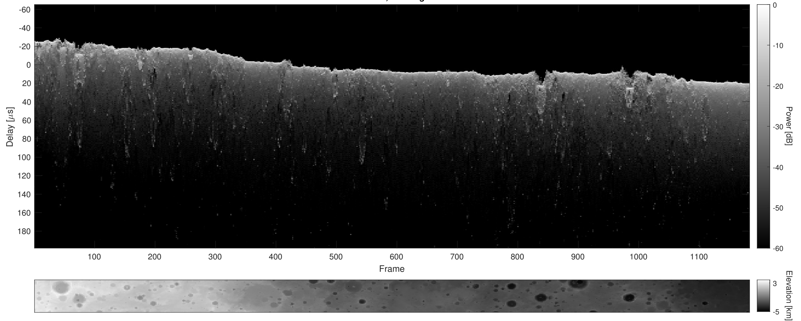
Orbit 8240, Cluttergram
