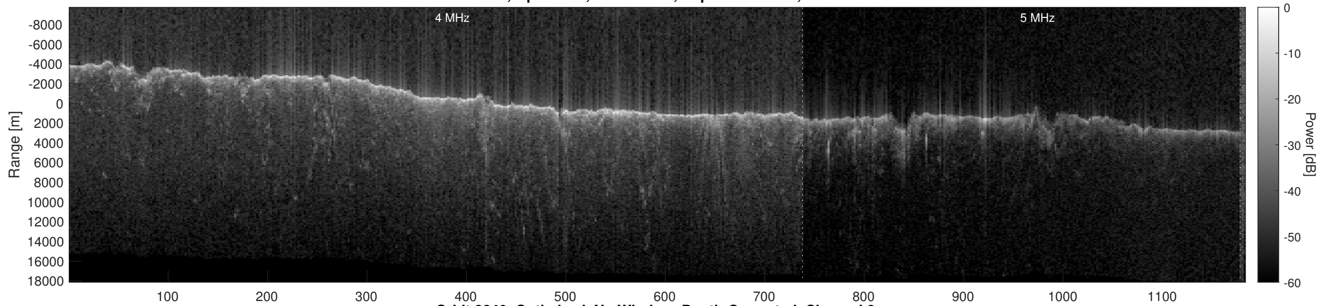
Orbit 8240, Optimized, No Window, Depth-Corrected, Channel 2
