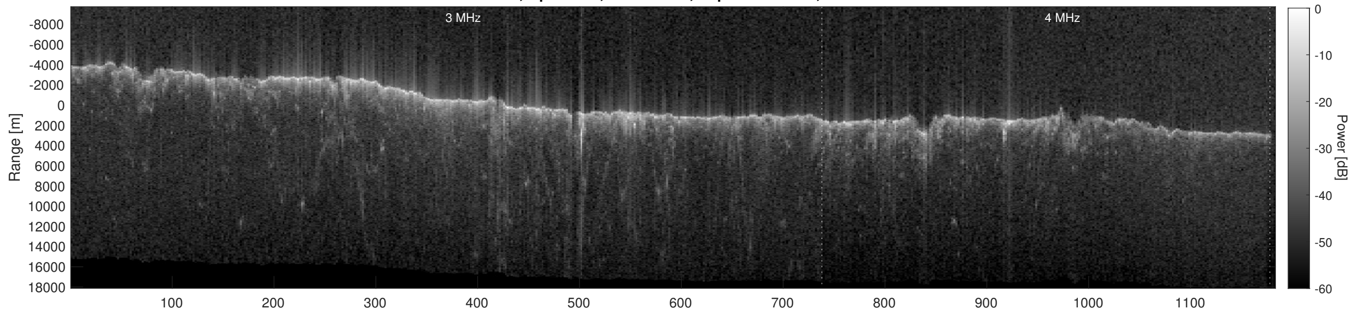
Orbit 8240, Depth-Corrected Cluttergram
