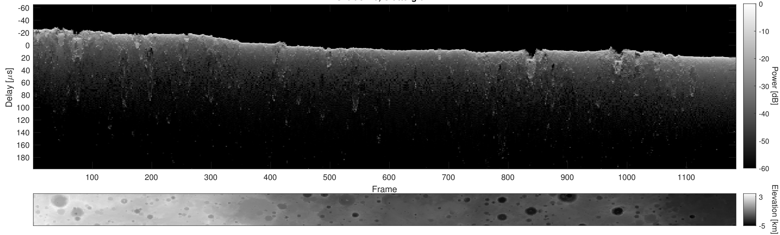
Orbit 8240, Cluttergram
