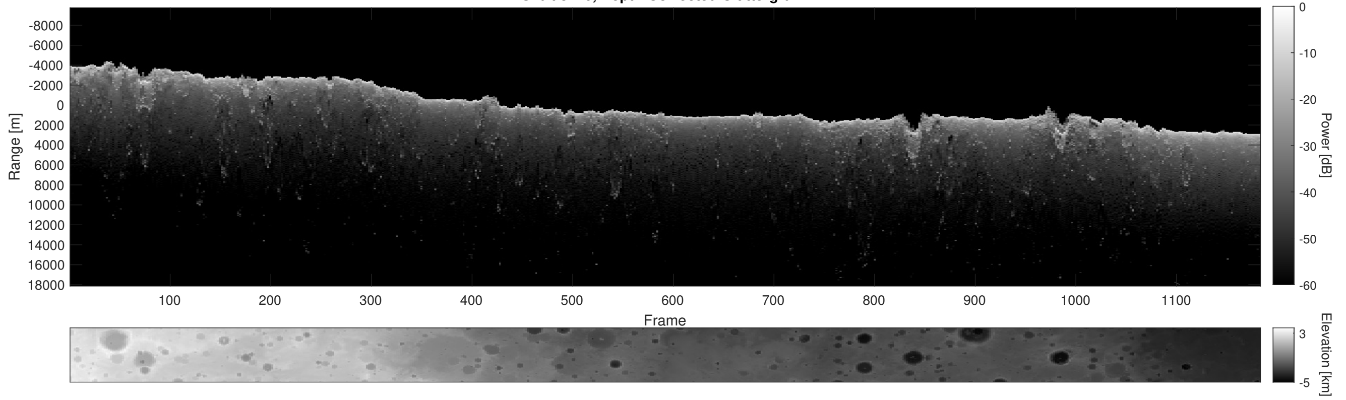
Orbit 8240, Depth-Corrected Cluttergram
