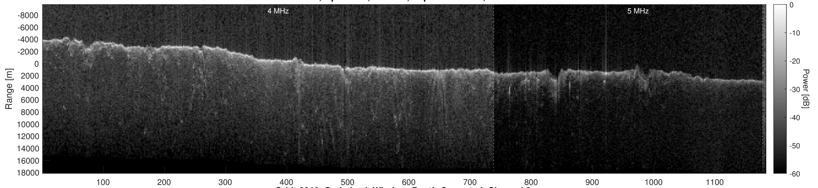
Orbit 8240, Optimized, Window, Depth-Corrected, Channel 2
