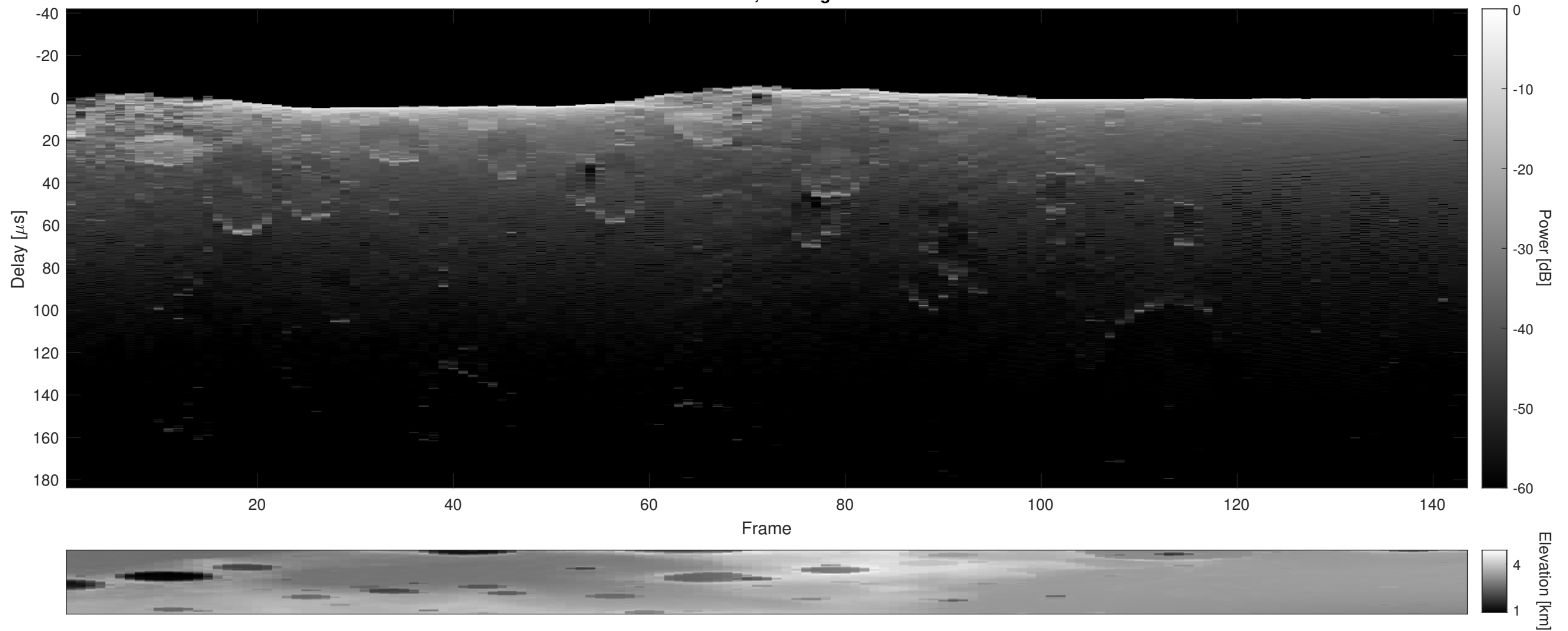
Orbit 8241, Cluttergram
