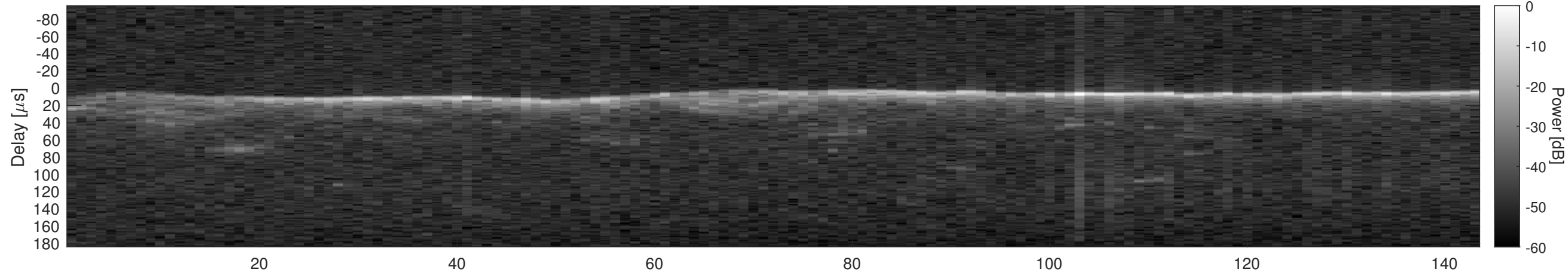
Orbit 8241, Window, Channel 2, Chapman
