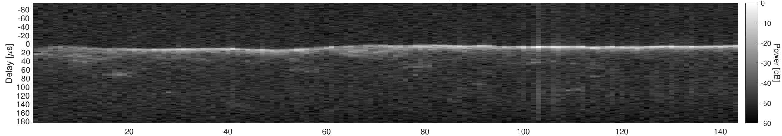
Orbit 8241, Window, Channel 2, Optimized
