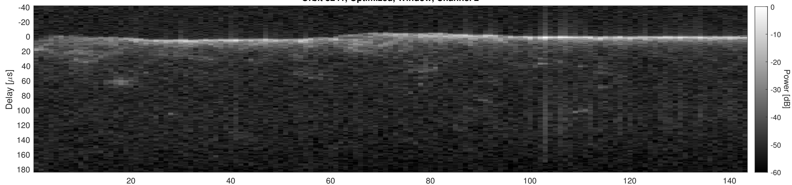
Orbit 8241, Cluttergram
