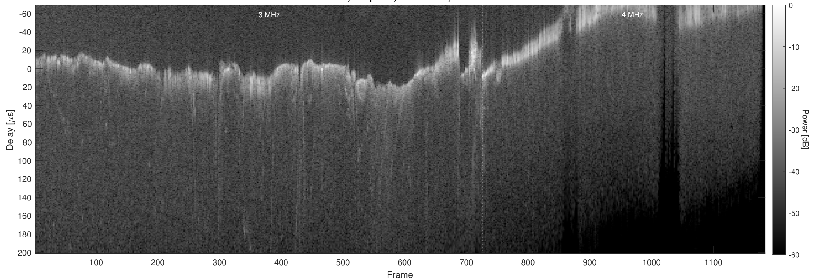
Orbit 8242, Chapman, No Window, Channel 2
