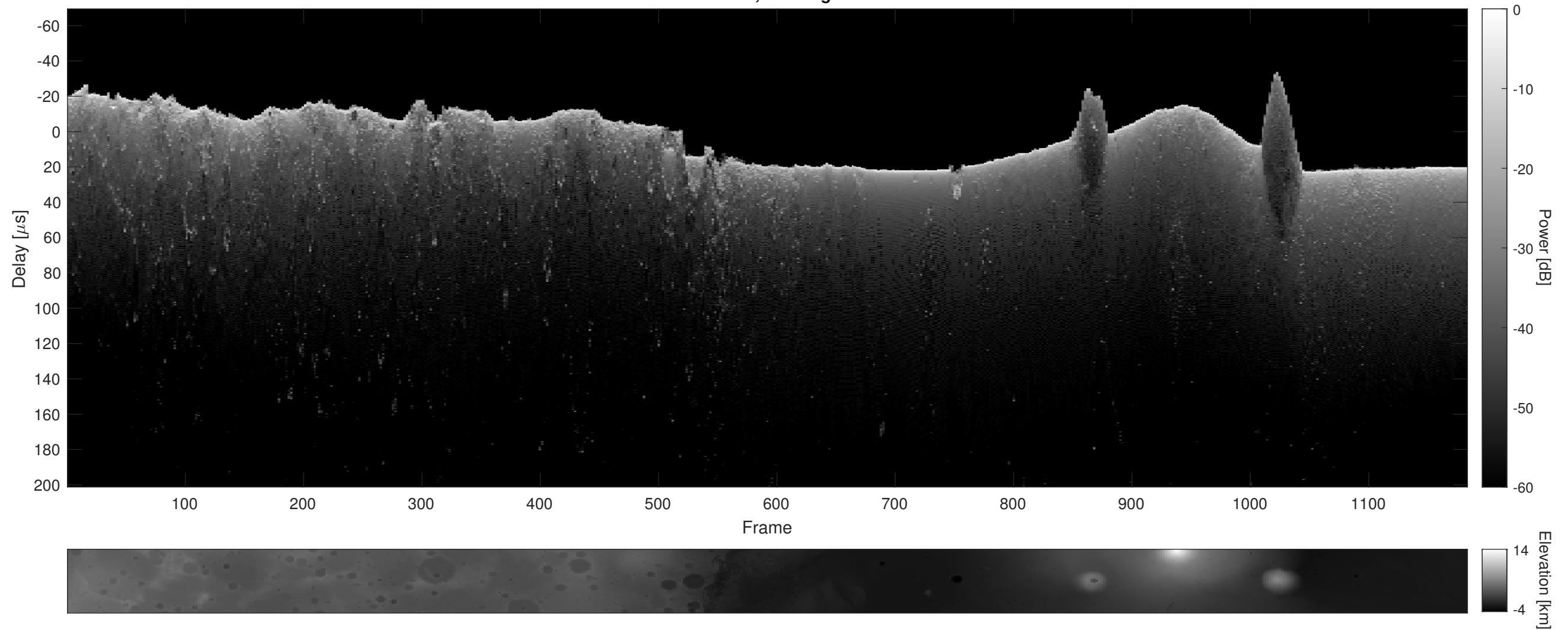
Orbit 8242, Cluttergram
