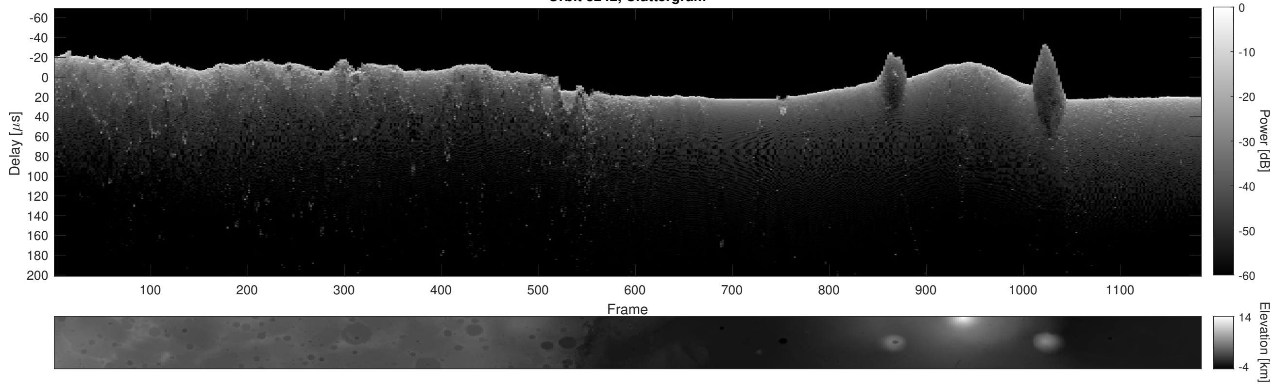
Orbit 8242, Cluttergram
