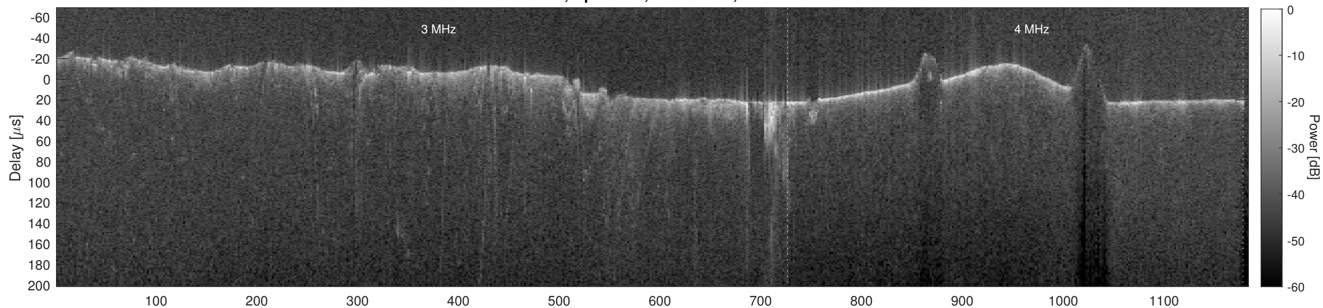
Orbit 8242, Cluttergram
