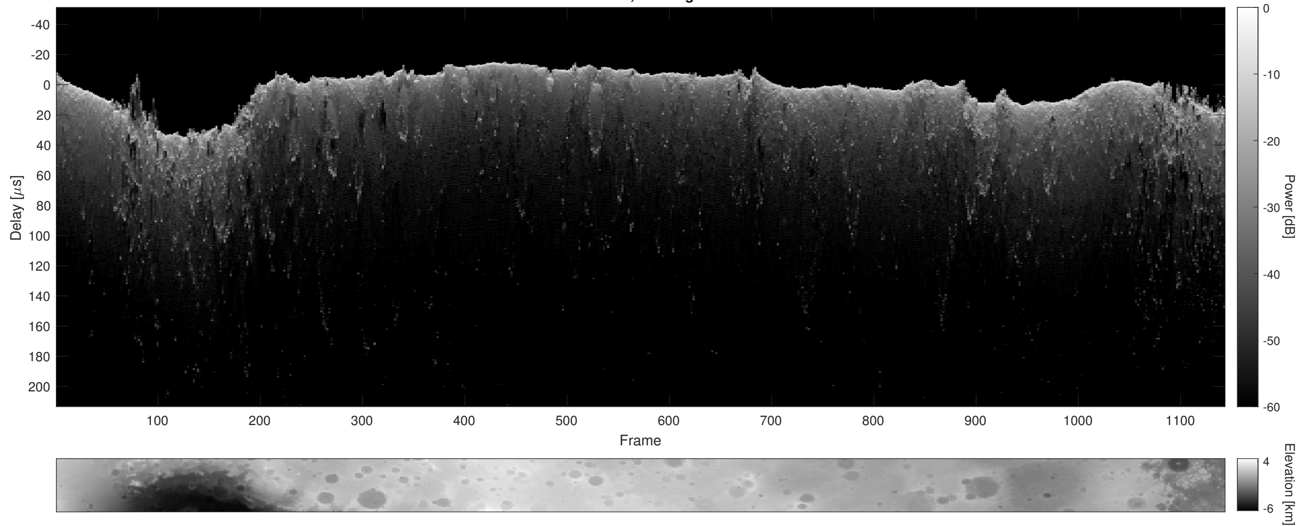
Orbit 8243, Cluttergram
