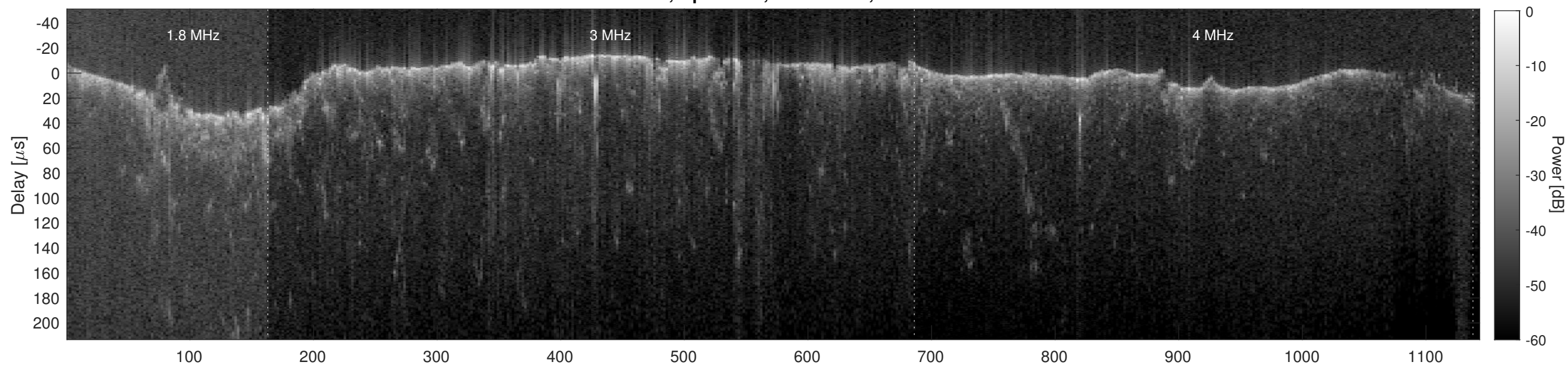
Orbit 8243, Cluttergram
