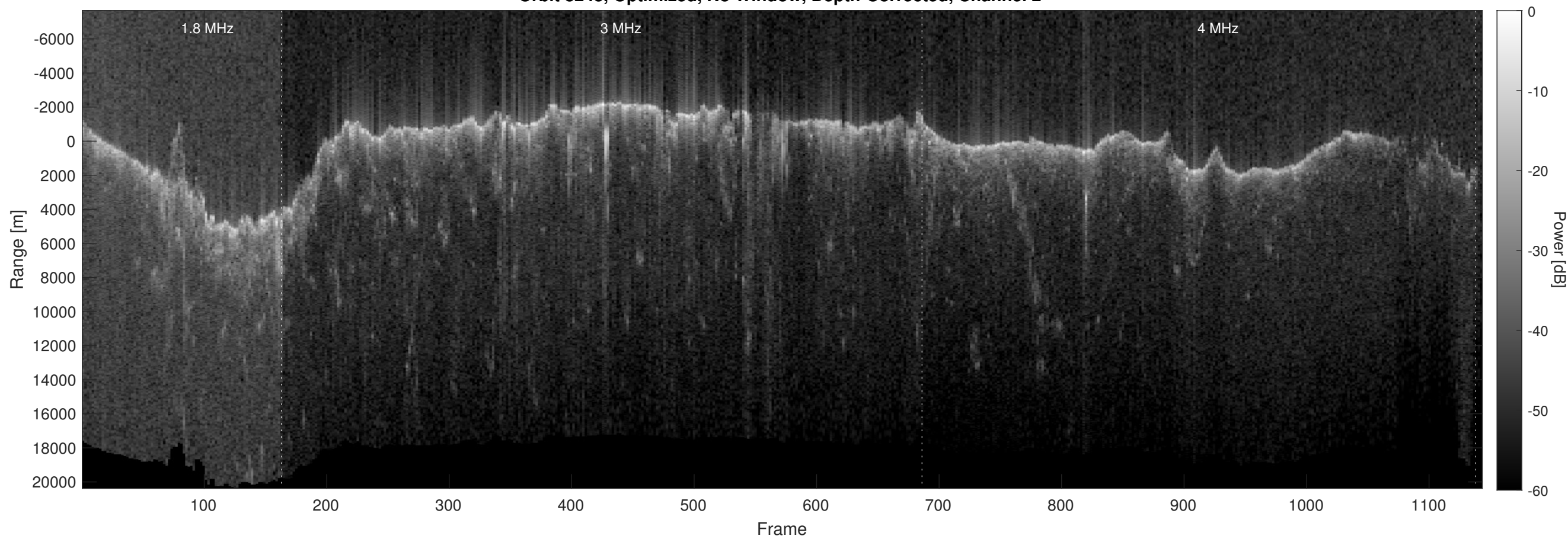
Orbit 8243, Optimized, No Window, Depth-Corrected, Channel 2
