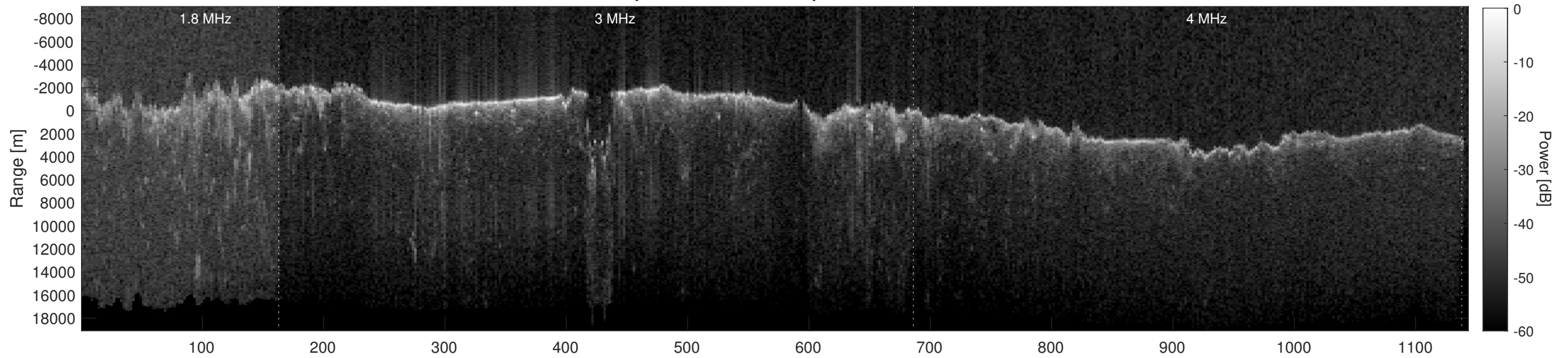
Orbit 8244, Depth-Corrected Cluttergram
