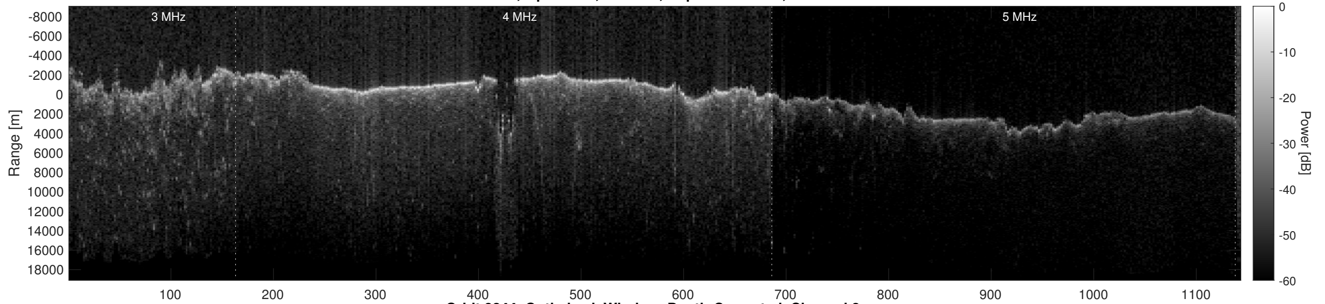
Orbit 8244, Optimized, Window, Depth-Corrected, Channel 2
