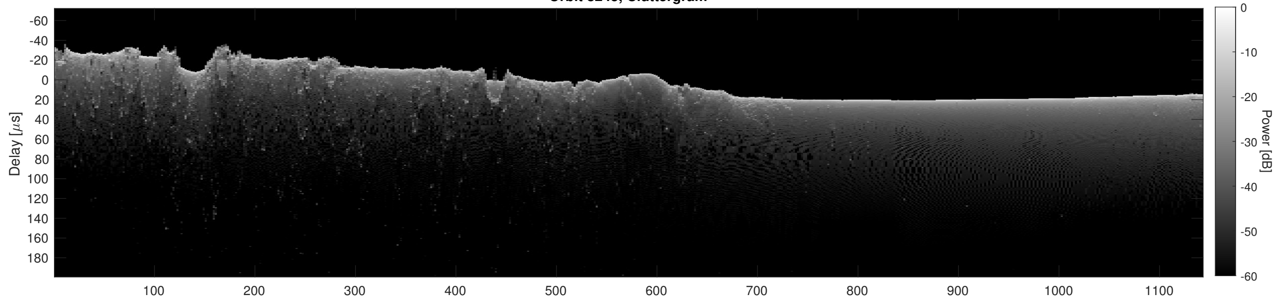
Orbit 8245, Cluttergram
