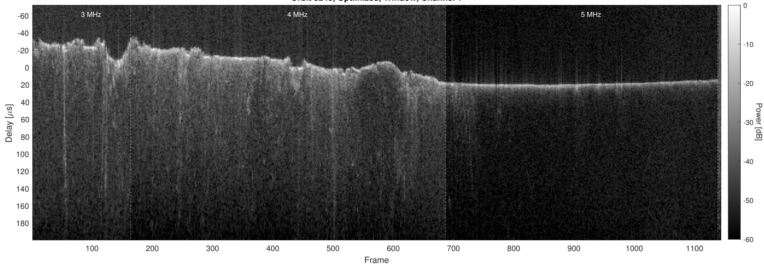
Orbit 8245, Optimized, Window, Channel 2
