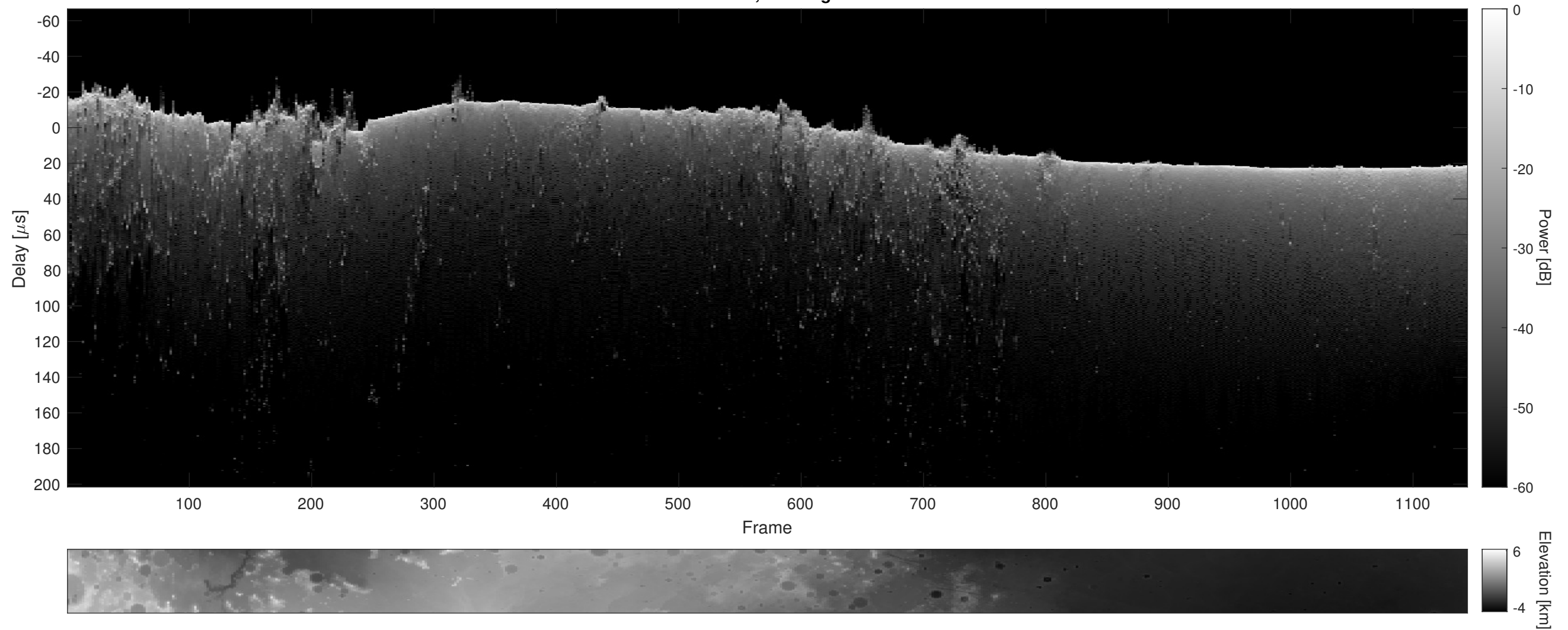
Orbit 8246, Cluttergram
