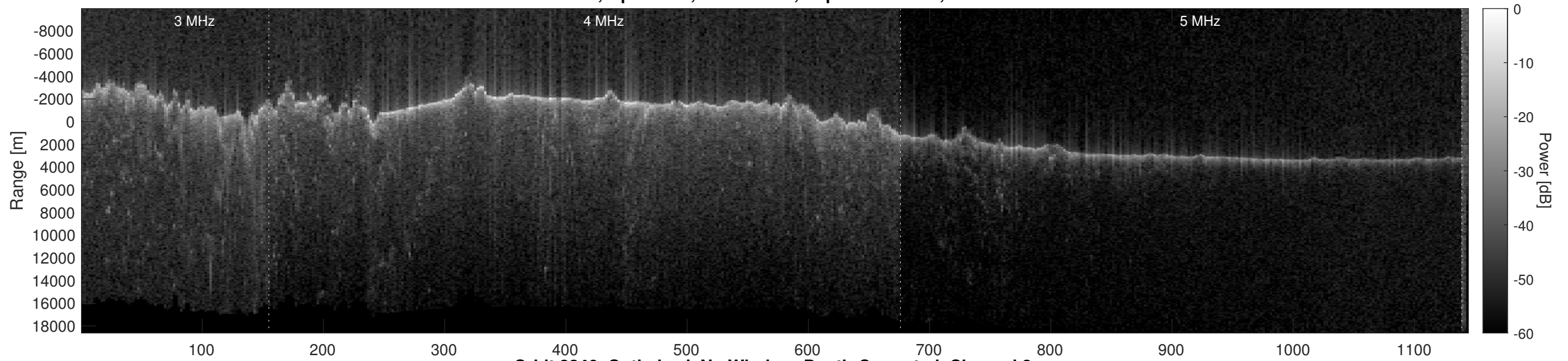
Orbit 8246, Optimized, No Window, Depth-Corrected, Channel 2
