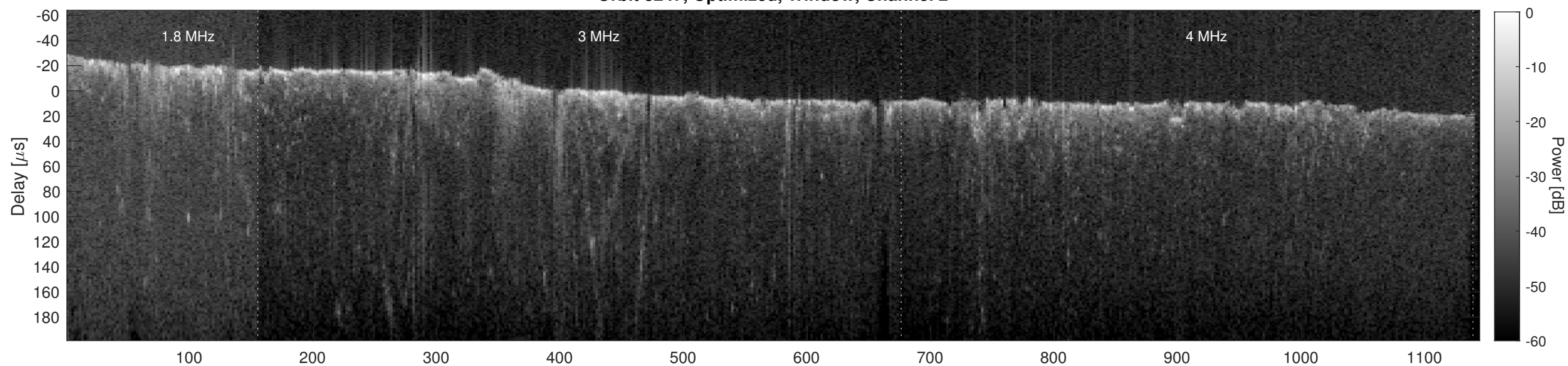
Orbit 8247, Cluttergram
