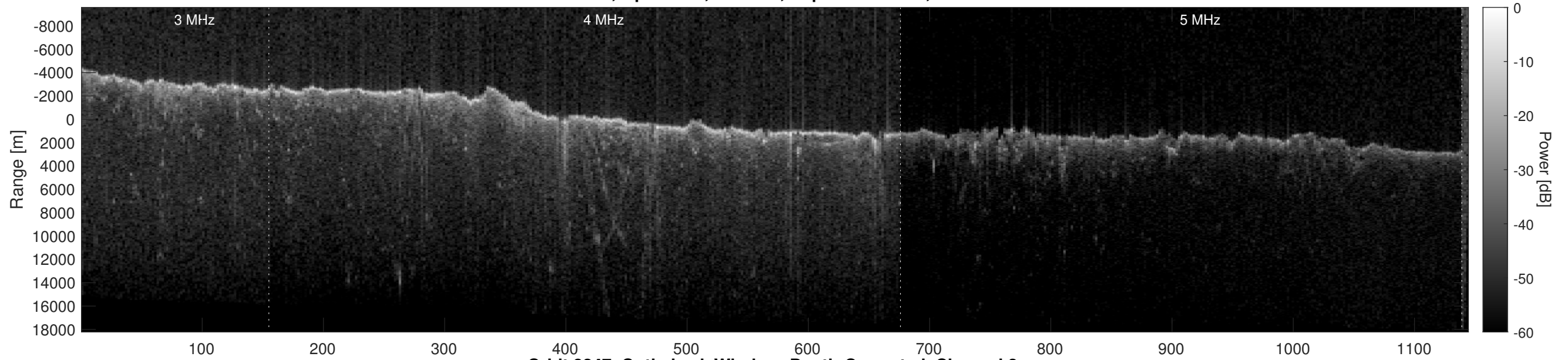
Orbit 8247, Optimized, Window, Depth-Corrected, Channel 2
