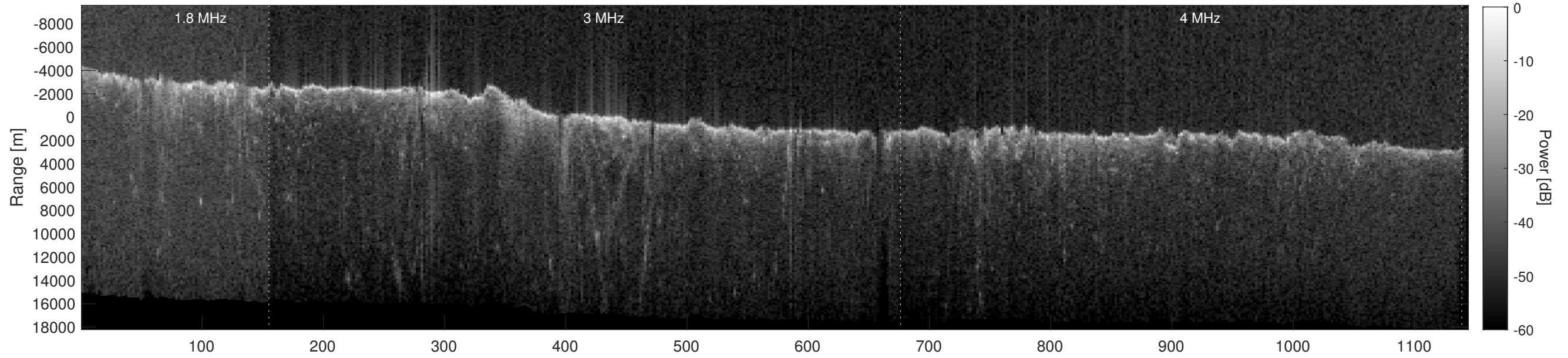
Orbit 8247, Depth-Corrected Cluttergram
