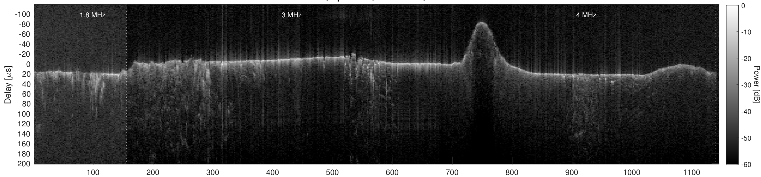
Orbit 8248, Cluttergram
